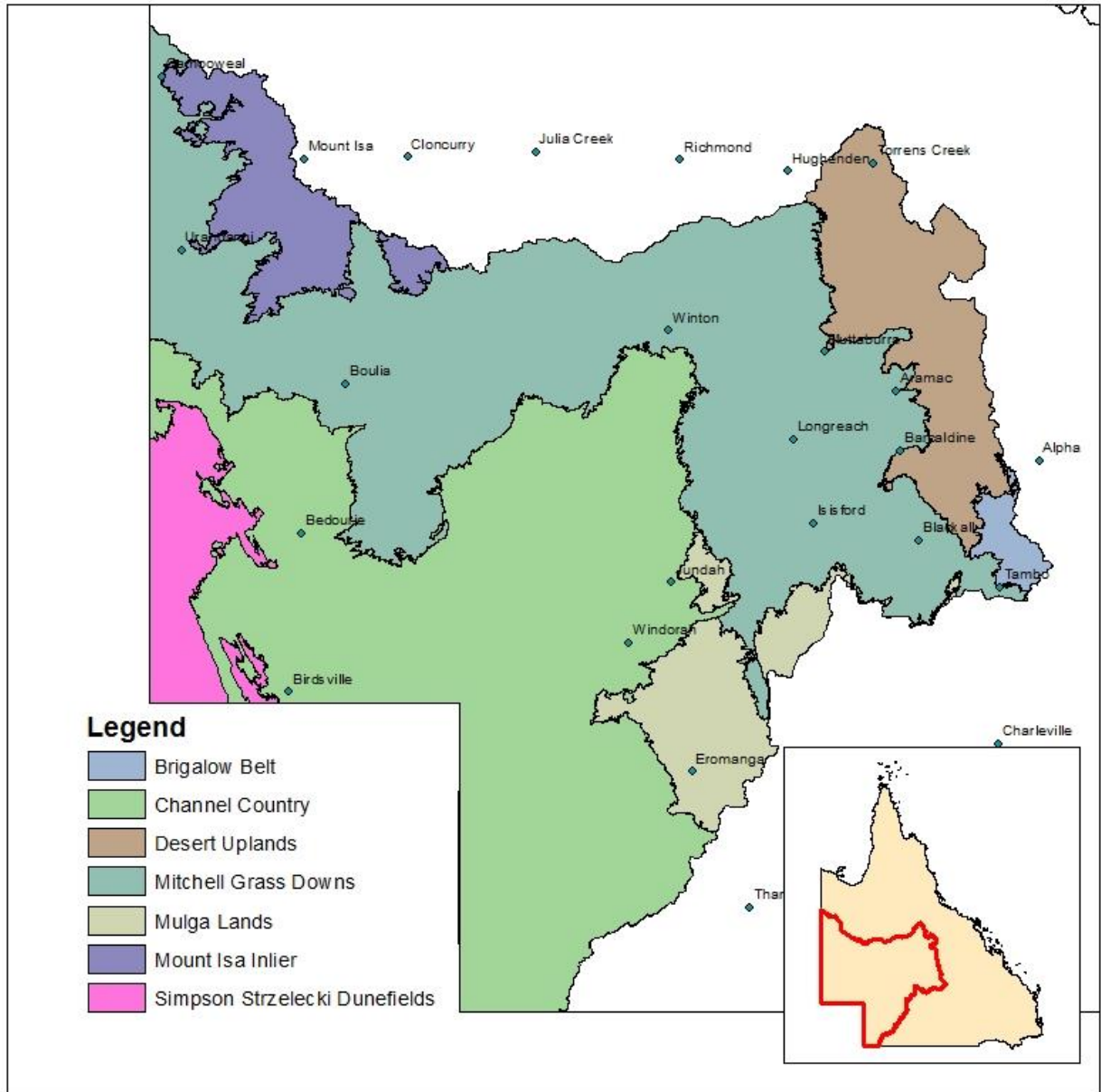
Map 3: Bioregions of the Desert Channels Region. (see the below box for a detailed description)
