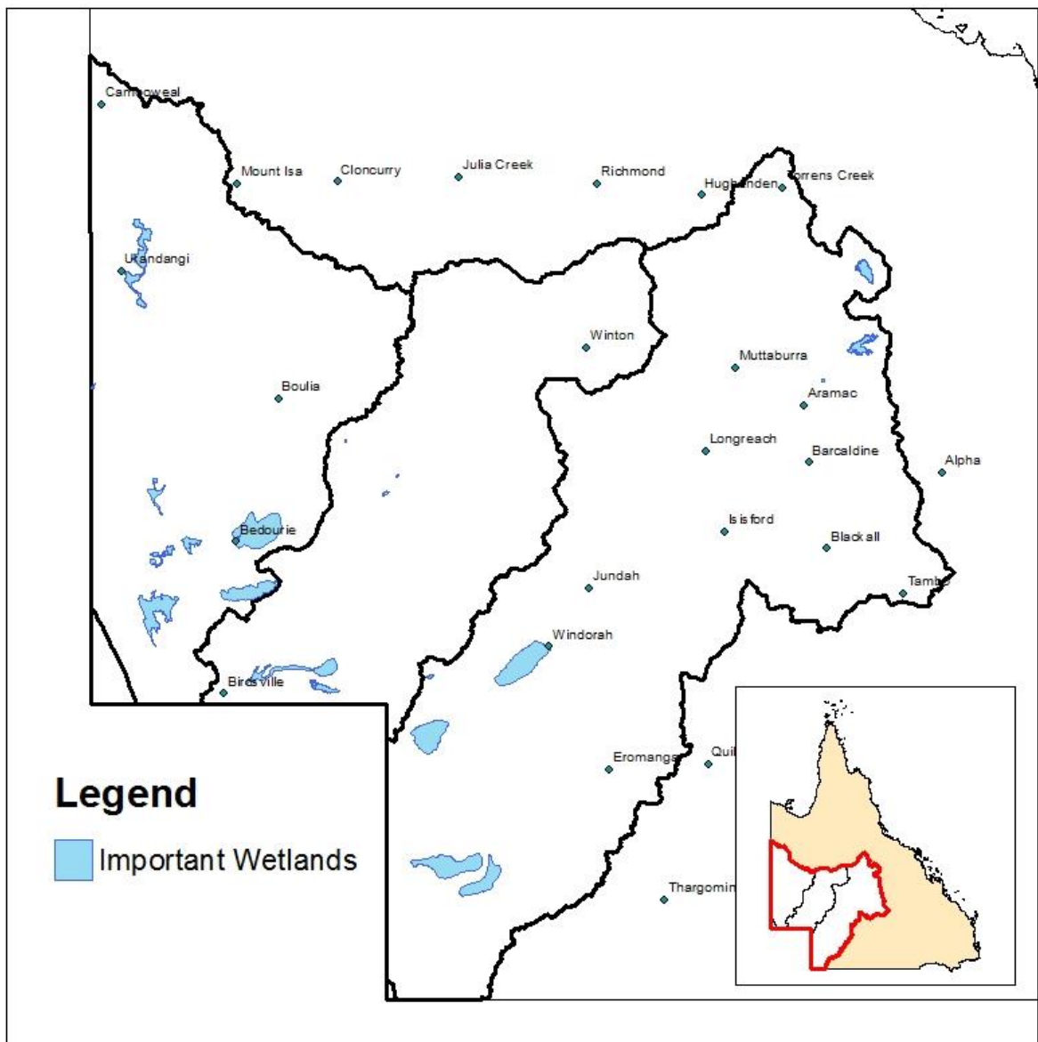
Map 2: Directory of Important Wetlands in the Desert Channels region. (see Appendix 3 for a full listing of the wetlands)
